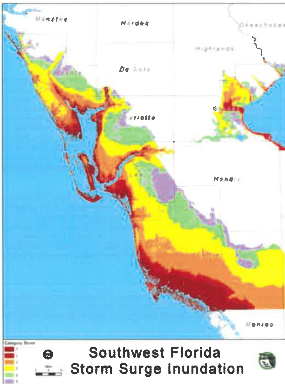
Figure 7 Storm Surge for the Southwest Region
